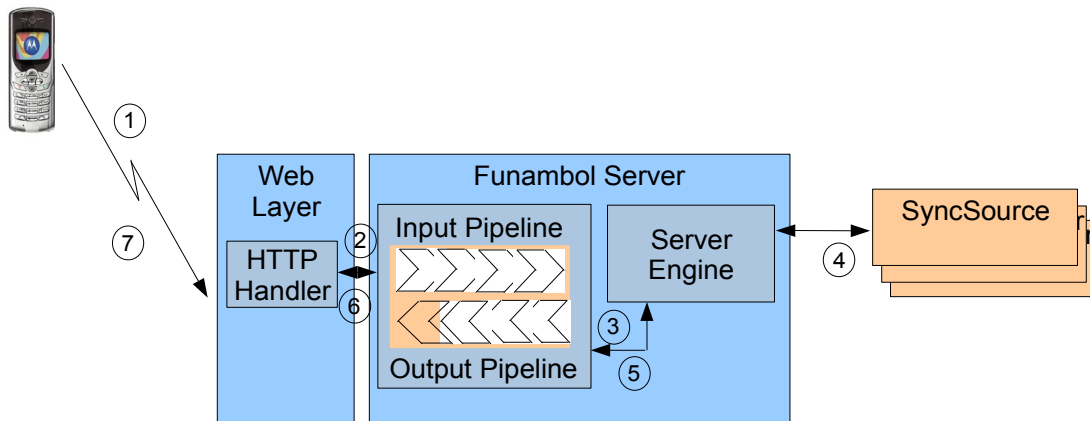
Figure 3: Execution flow of an OMA DS request
